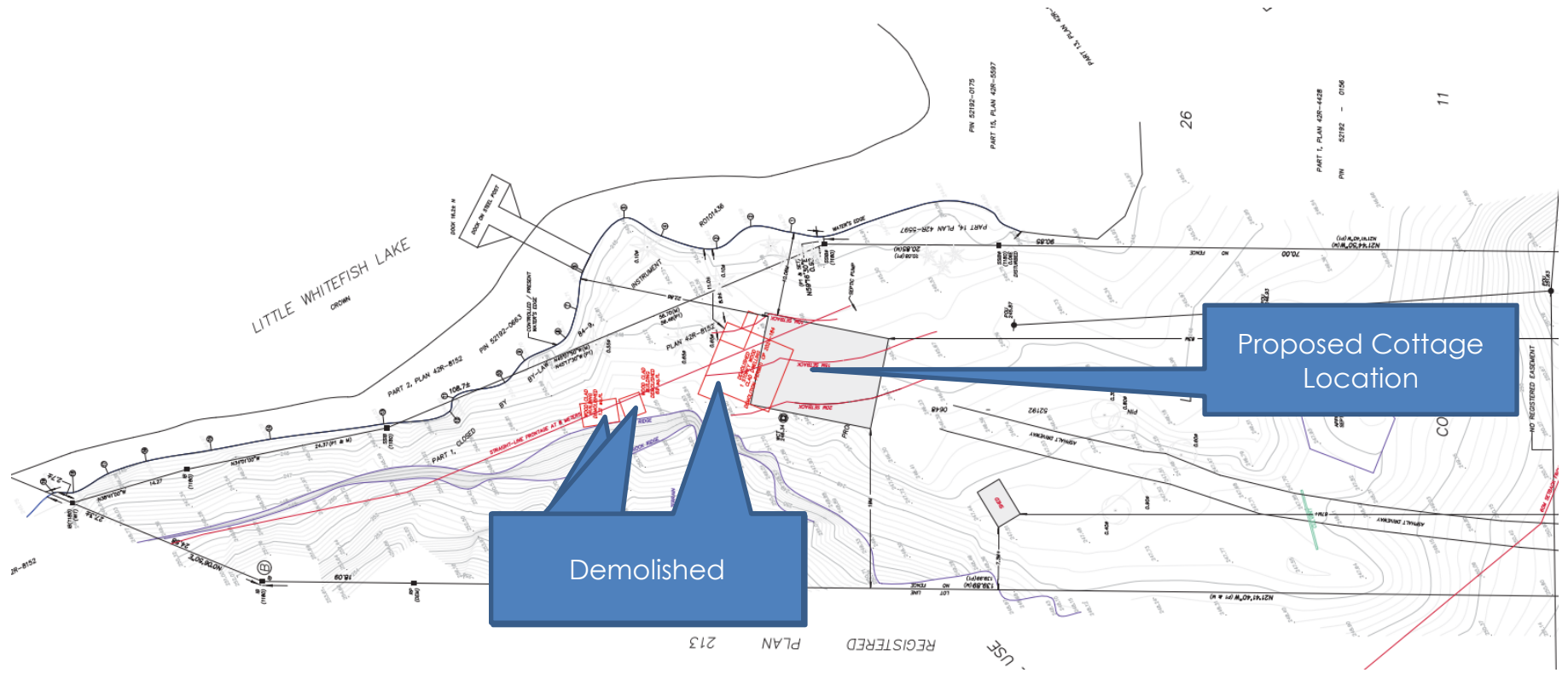
Figure 2: Proposed Site Plan (Excerpt)
